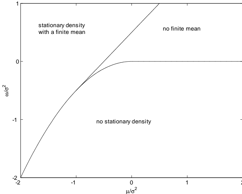
FIGURE II Conditions for Stationarity and a Finite Mean
