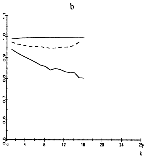
FIG. 3.—MSE decomposition: output prices. MSE ratio estimates and 95 percent confidence intervals: MSE(x_{t+k} - x_t) / [MSE(x_{t+k} - x_t) + MSE(y_{t+k} - y_t)] . a , Canadian/U.S. output price real exchange rate, 1960–89. b , Japanese/U.S. output price real exchange rate, 1970–89. c , Germany, Denmark, Finland, France, and Norway, 1960–89.
